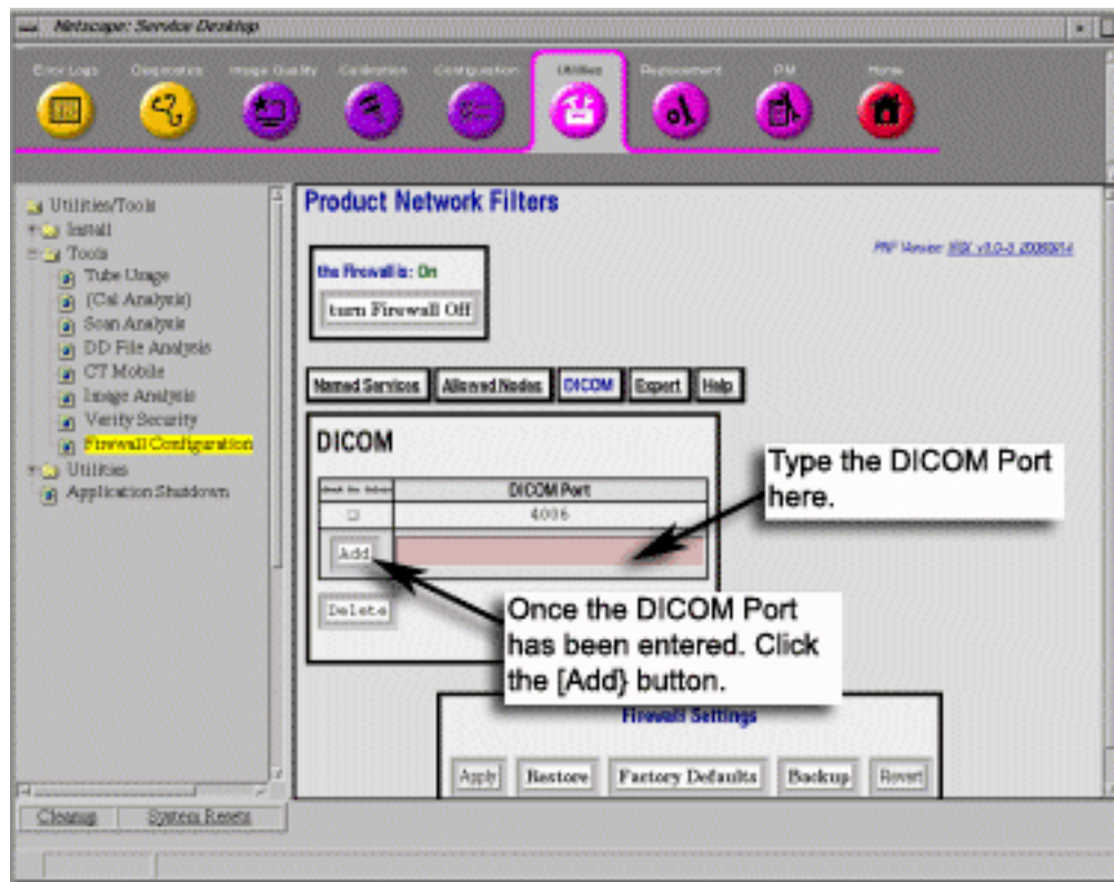
Illustration 7: DICOM Tab
