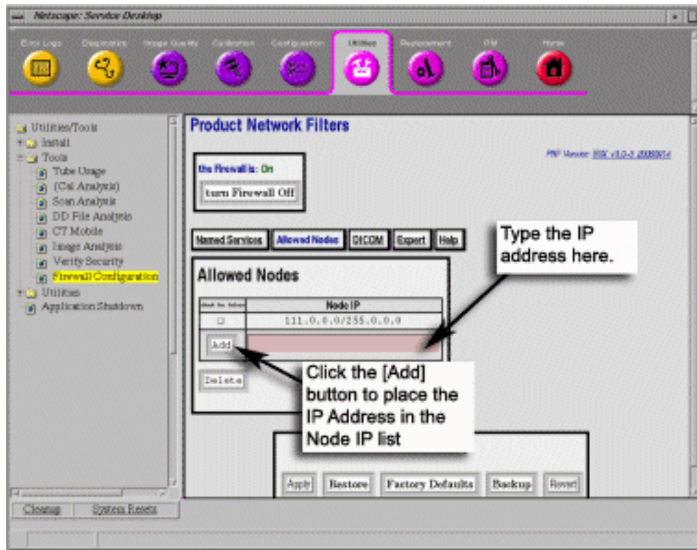
Illustration 6: Allowed Nodes
