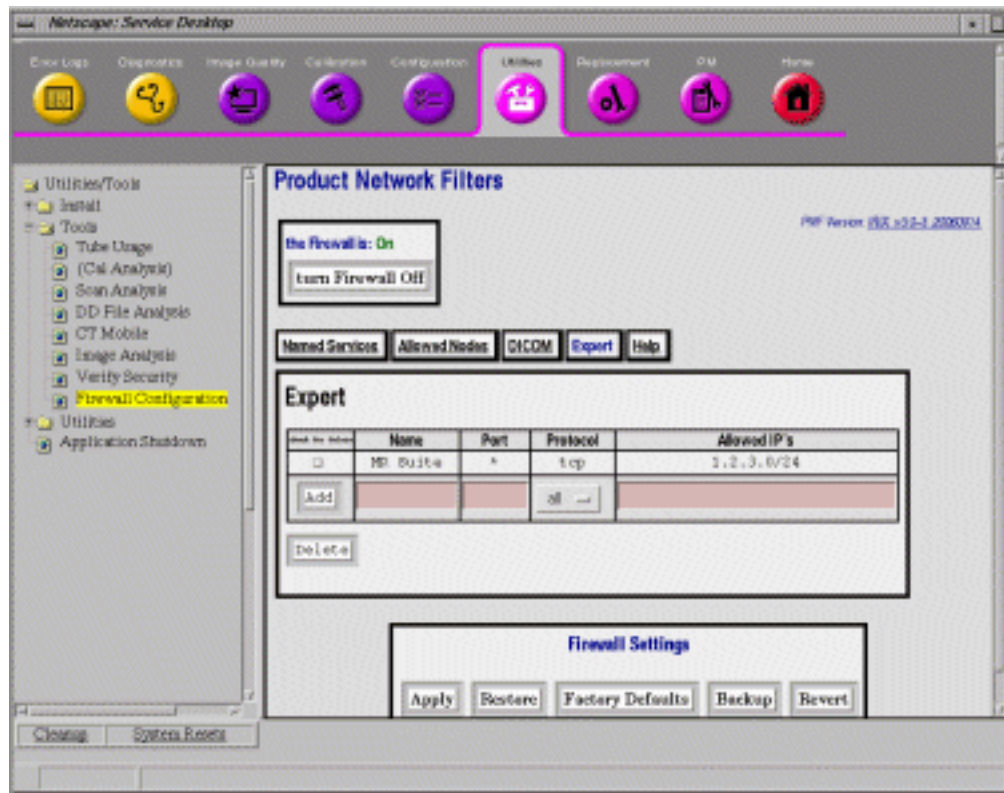
Illustration 8: Expert Tab
